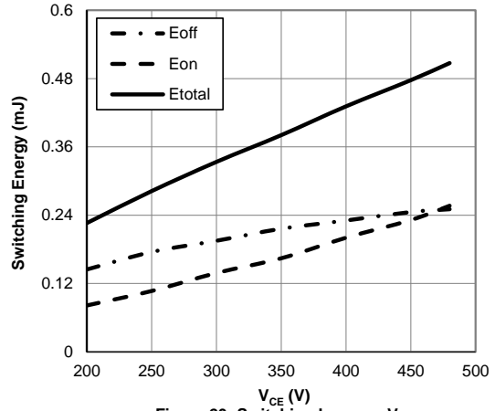
Figure 20: Switching Loss vs. V_{CE} ( T_j=175^\circ C, V_{GE}=15V, I_C=10A, R_g=30\Omega )
