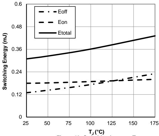
Figure 19: Switching Loss vs. T_j ( V_{GE}=15V, V_{CE}=400V, I_C=10A, R_g=30\Omega )
